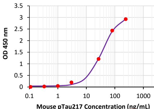
Fig.3 Mouse pTau217 Standard Curve
