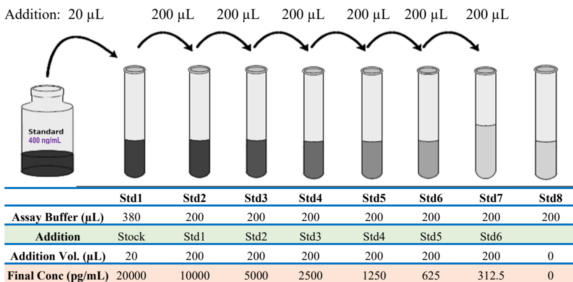
Fig.2 Diagram for Human Beta-Catenin standard preparation
