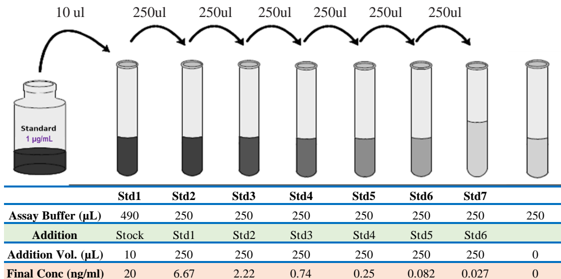
Fig.2 Diagram for Human IgG standard preparation
