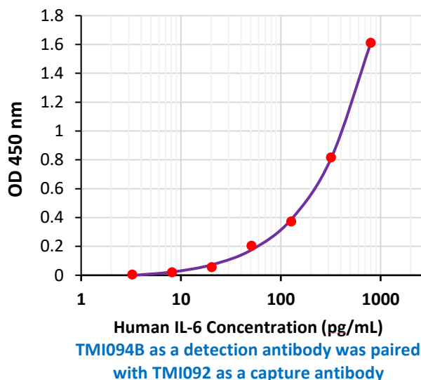
Fig.1 Human IL-6 Standard Curve
