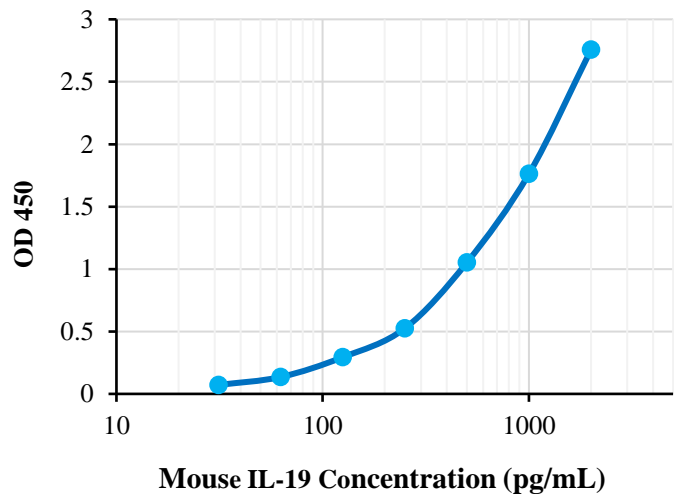
Fig.3 Mouse IL-19 Standard Curve
